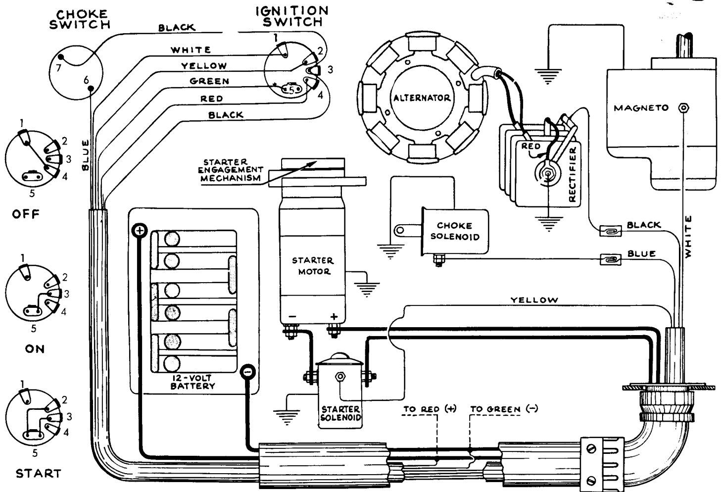
FIGURE 4. Mark 55E and Mark 50E Wiring Diagram (Positive Ground)
