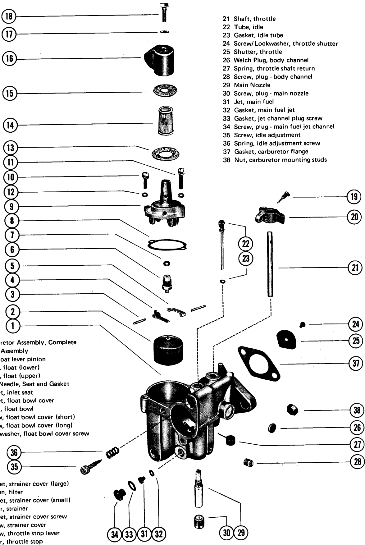
Figure 6. Pressure Type Carburetor
