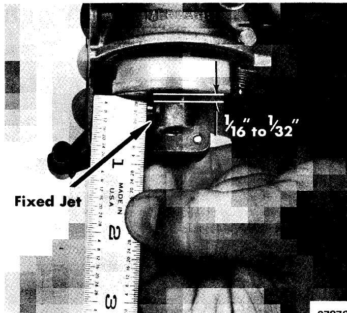
Figure 6. Float Drop Adjustment
