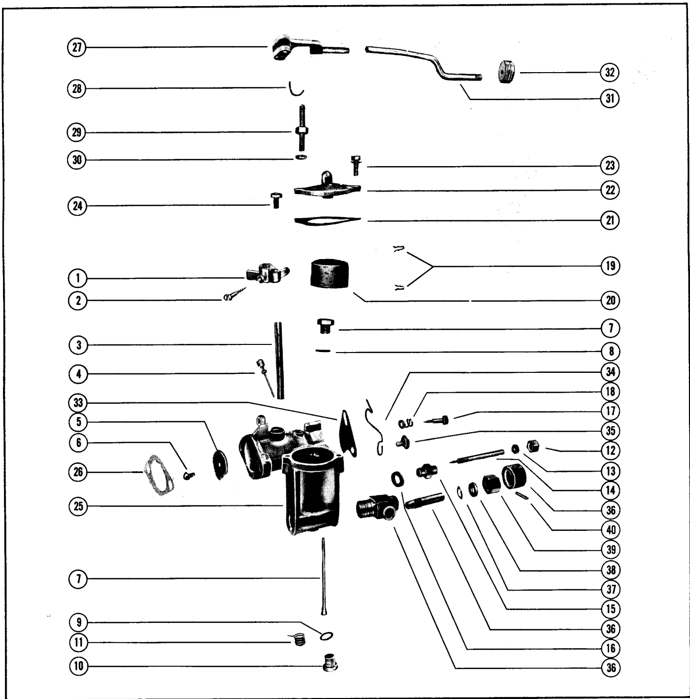
Figure 7. Gravity Feed Carburetor, Shut-Off Valve and Choke
