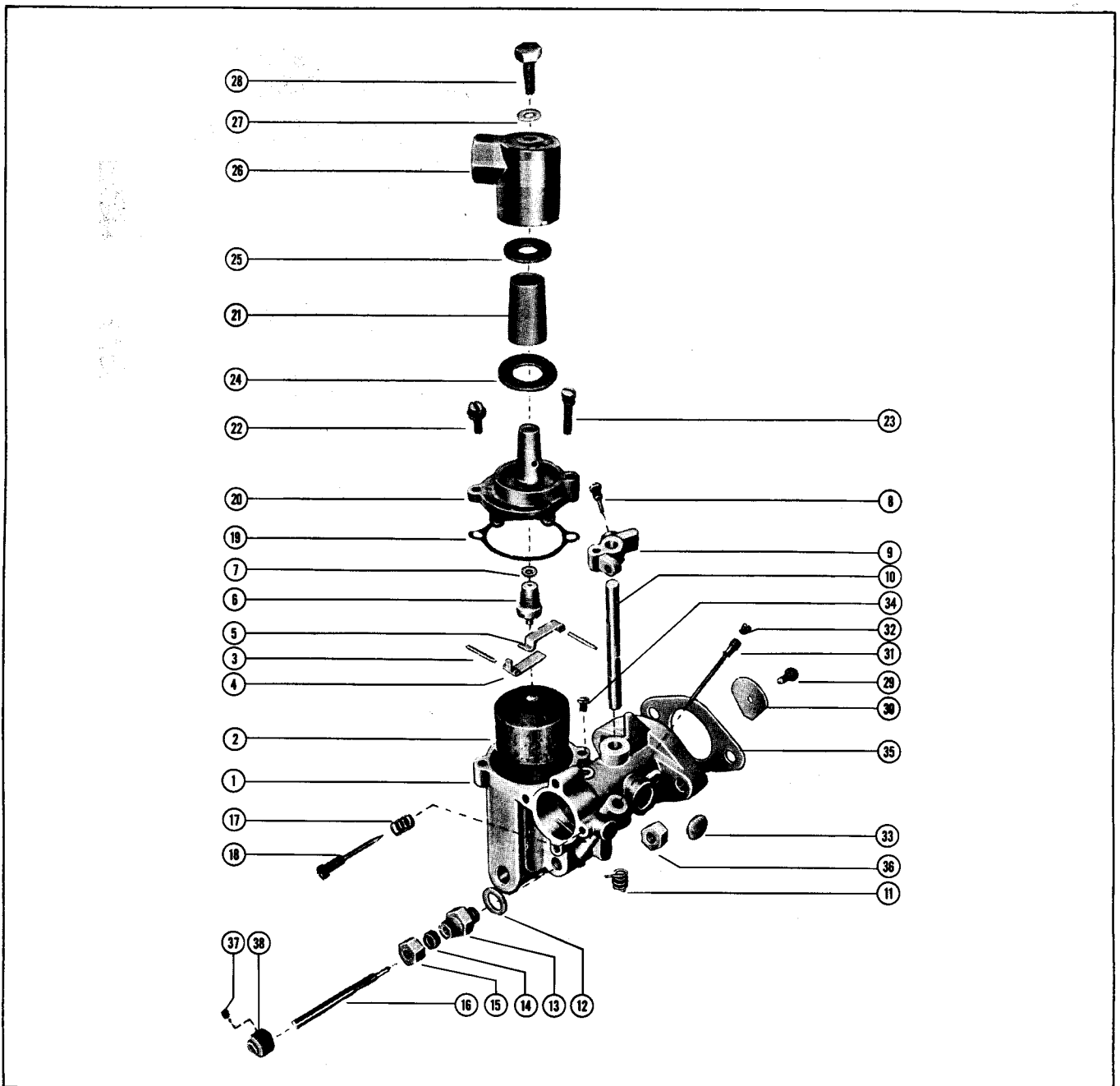
Figure 6. Pressure Feed Carburetor
